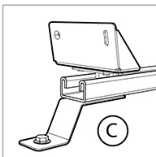
C: Existing Rail Hardware (alt.)
